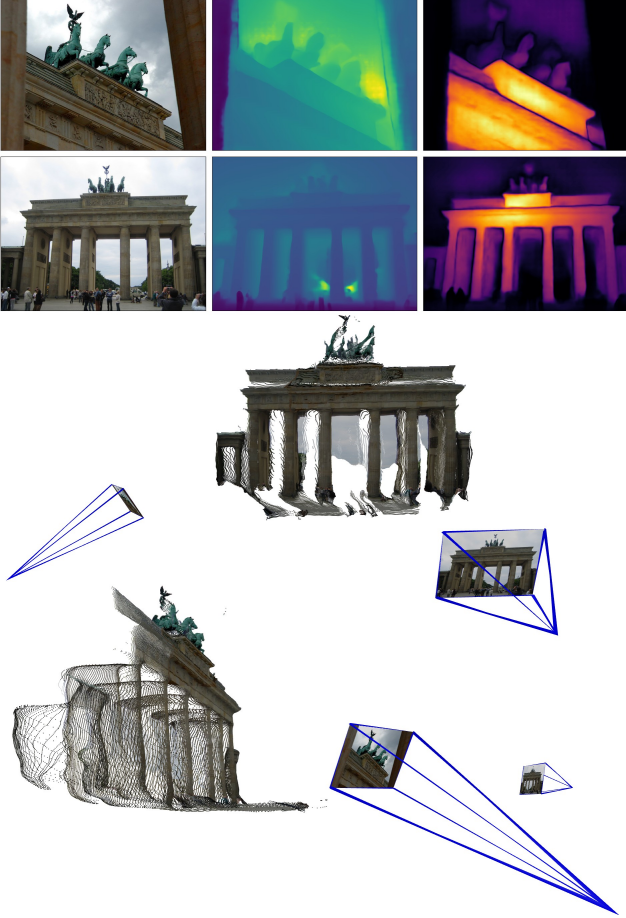
Figure 4. Example of 3D reconstruction of an unseen MegaDepth scene from two images (top-left). Note this is the raw output of the network , i.e. we show the output depthmaps (top-center, see Eq. (8)) and confidence maps (top-right), as well as two different viewpoints on the colored pointcloud (middle and bottom). Camera parameters are recovered from the raw pointmaps , see Sec. 3.3 in the main paper. DUS3R handles strong viewpoint and focal changes without apparent problems
